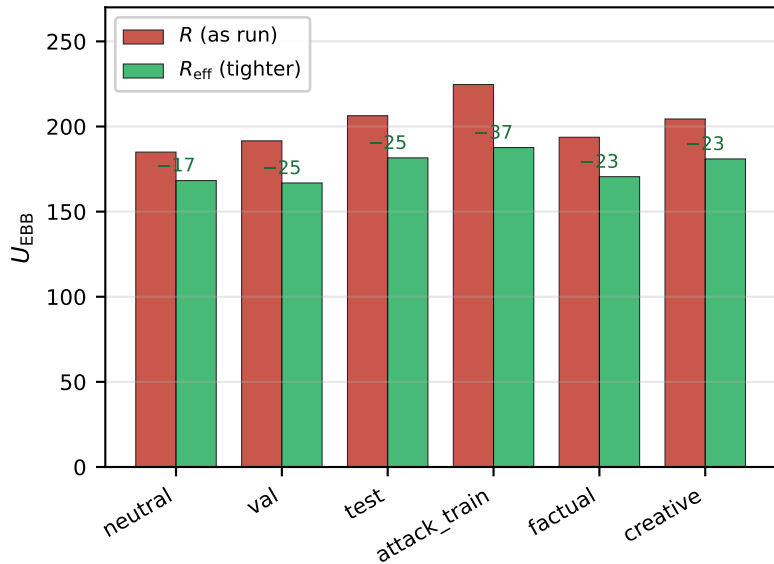
k = 3 ( K = 600 )
