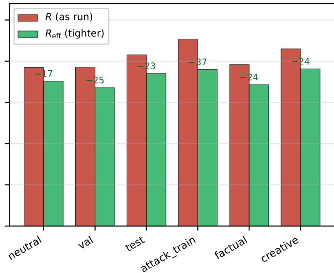
k = 5 ( K = 1000 )
