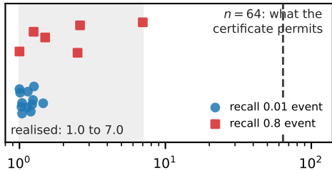
realised amplification at n = 64 , twelve contaminated anchors
