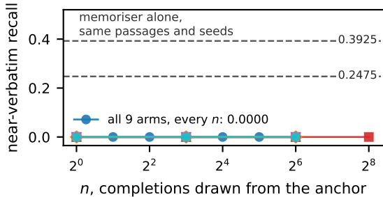
(a) selection reproduces nothing, at every n
