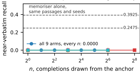
(a) selection reproduces nothing, at every n
