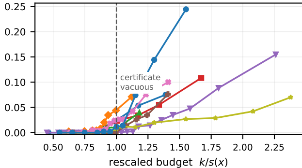
rescaled by the vacuity threshold
