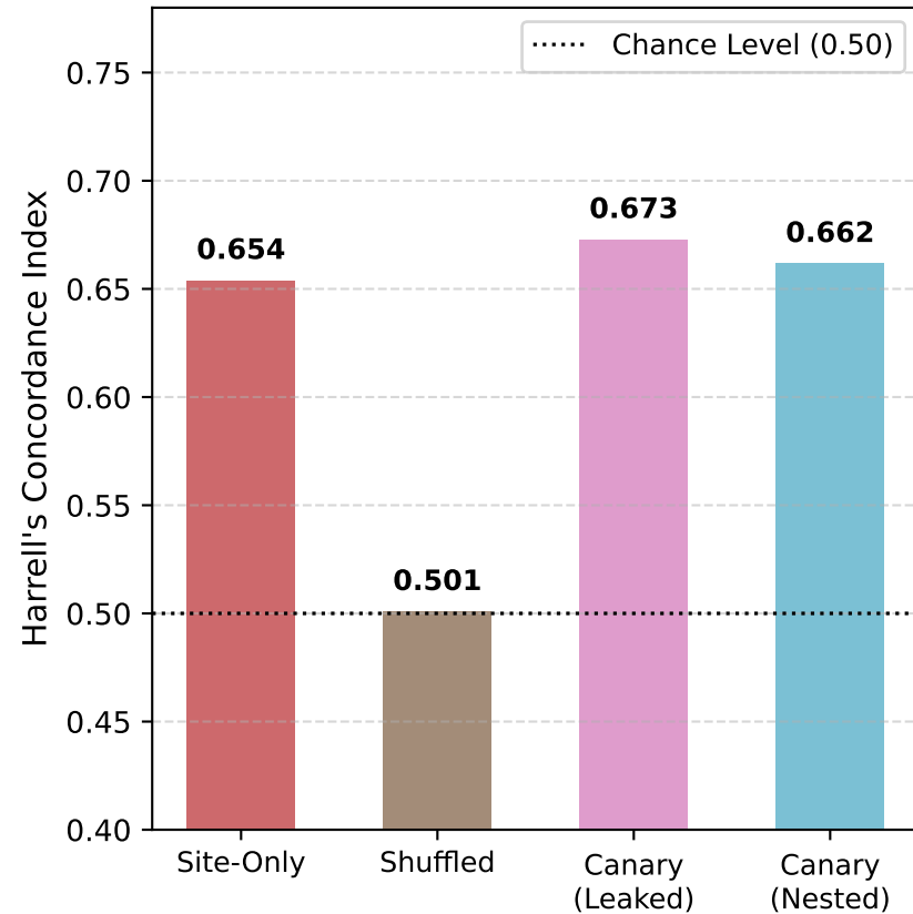
(A) Control & Diagnostic C-Indices
