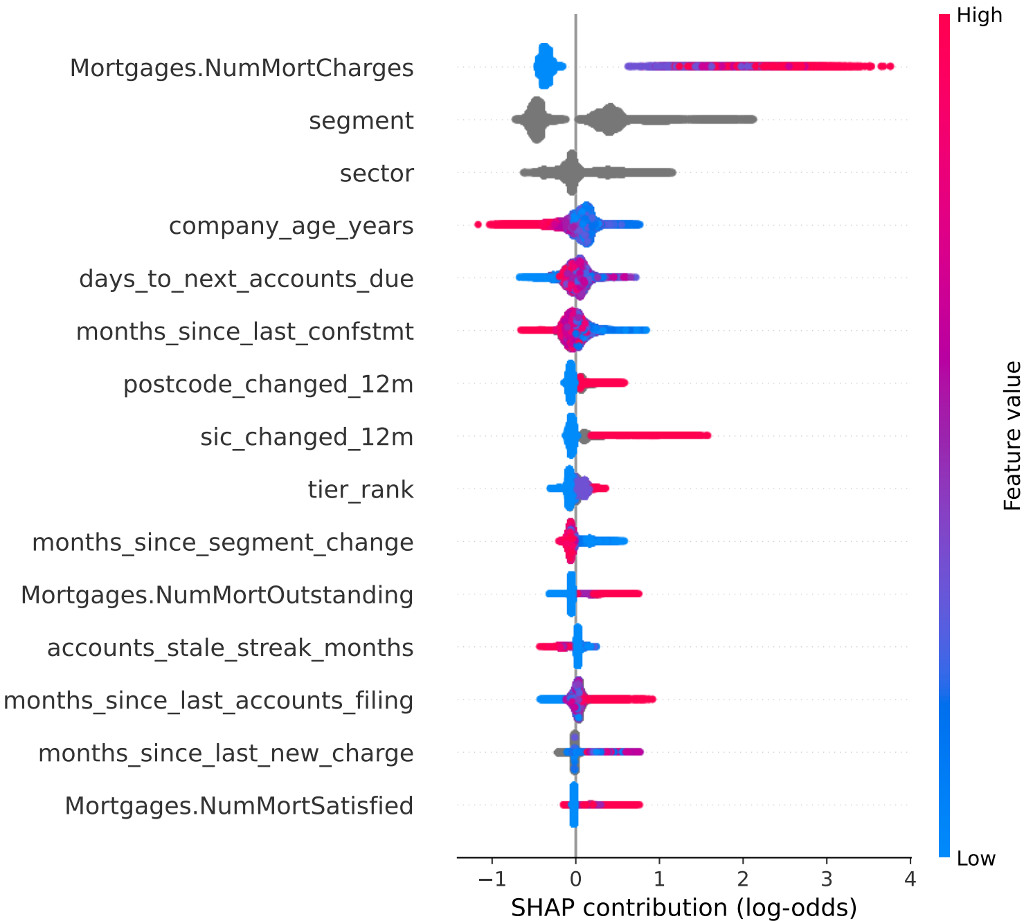
SHAP summary, lending (refactor_growthfix, 100,000 held-out rows)
