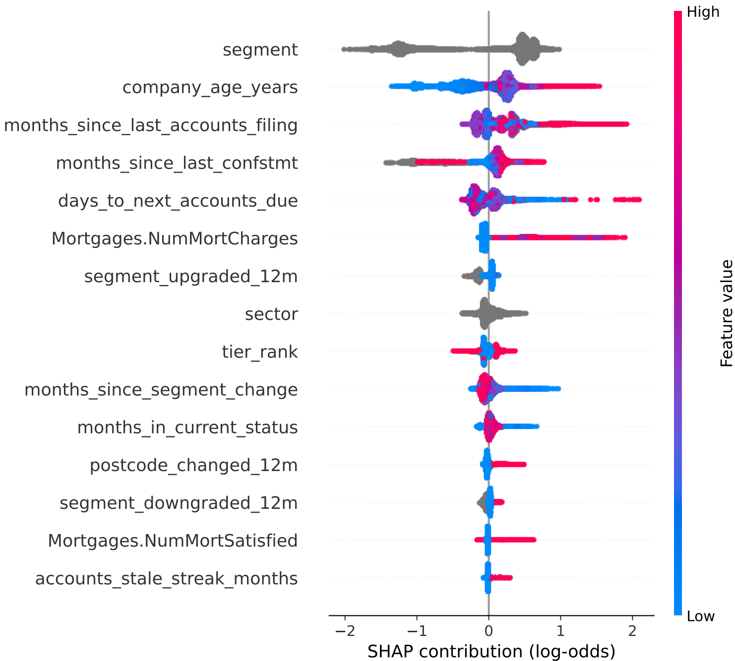
SHAP summary, insolvency (refactor_growthfix, 100,000 held-out rows)
