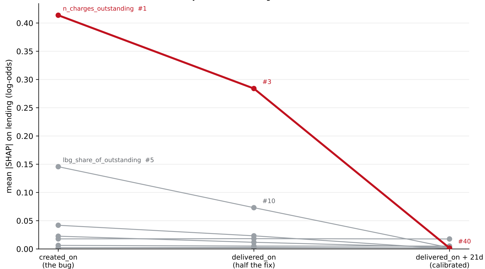
The leaking feature climbs to rank 1 and falls back when the gate is fixed lender-family features, lending, rank shown out of 54
