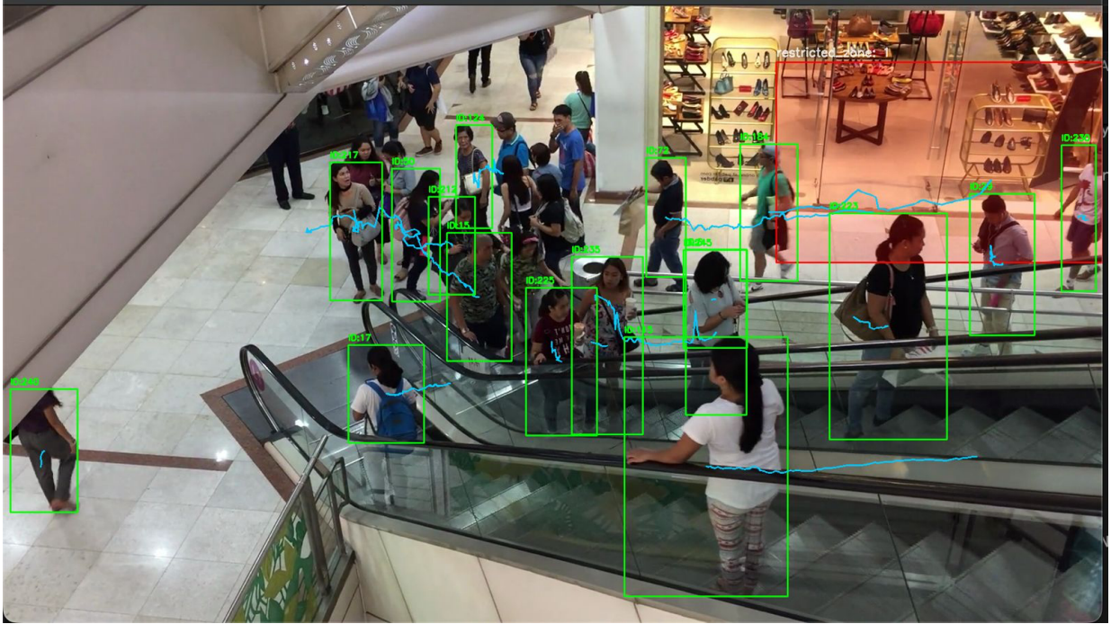
Fig 4.5: Sprint II exit demonstration – live YOLOv8 + ByteTrack output with persistent IDs, motion trails (cyan) and a restricted ROI overlay (red). Each box label shows ID:<n>.
