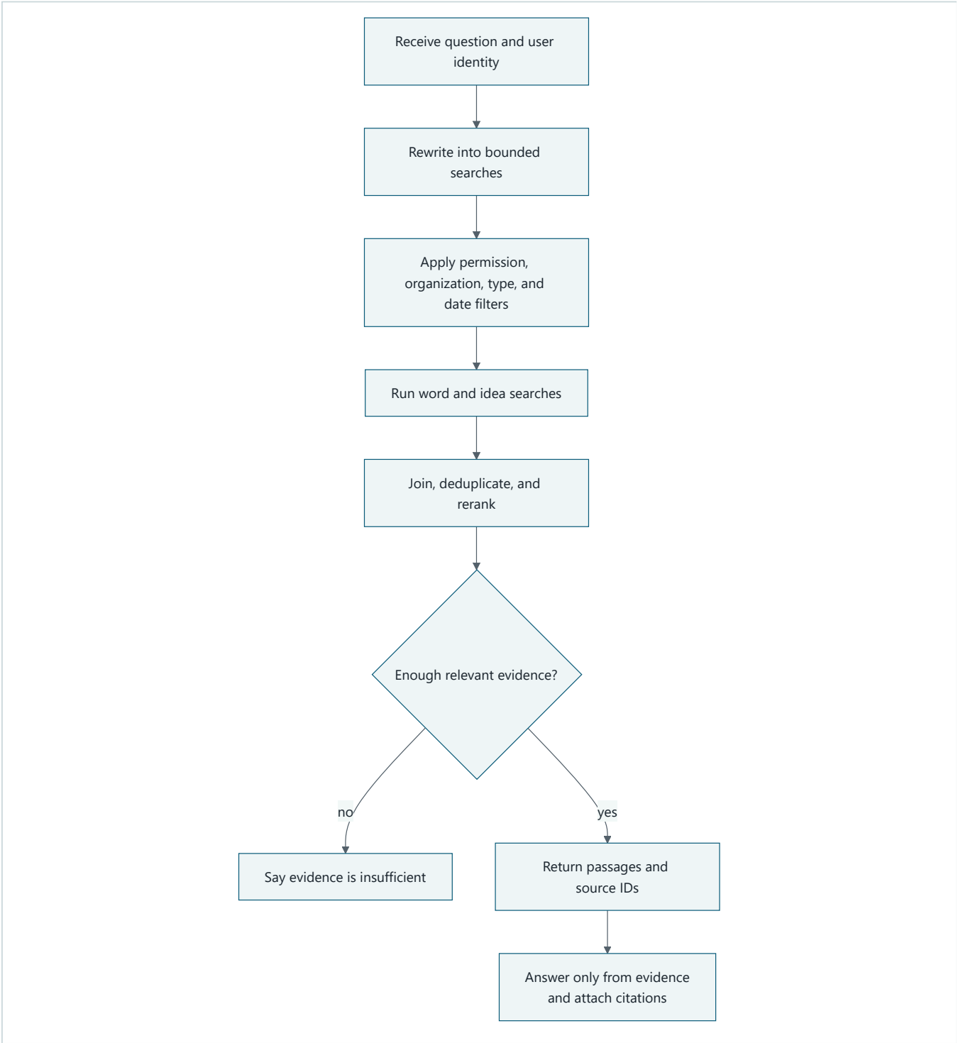
Visual 2: a boundary-first retrieval flow
