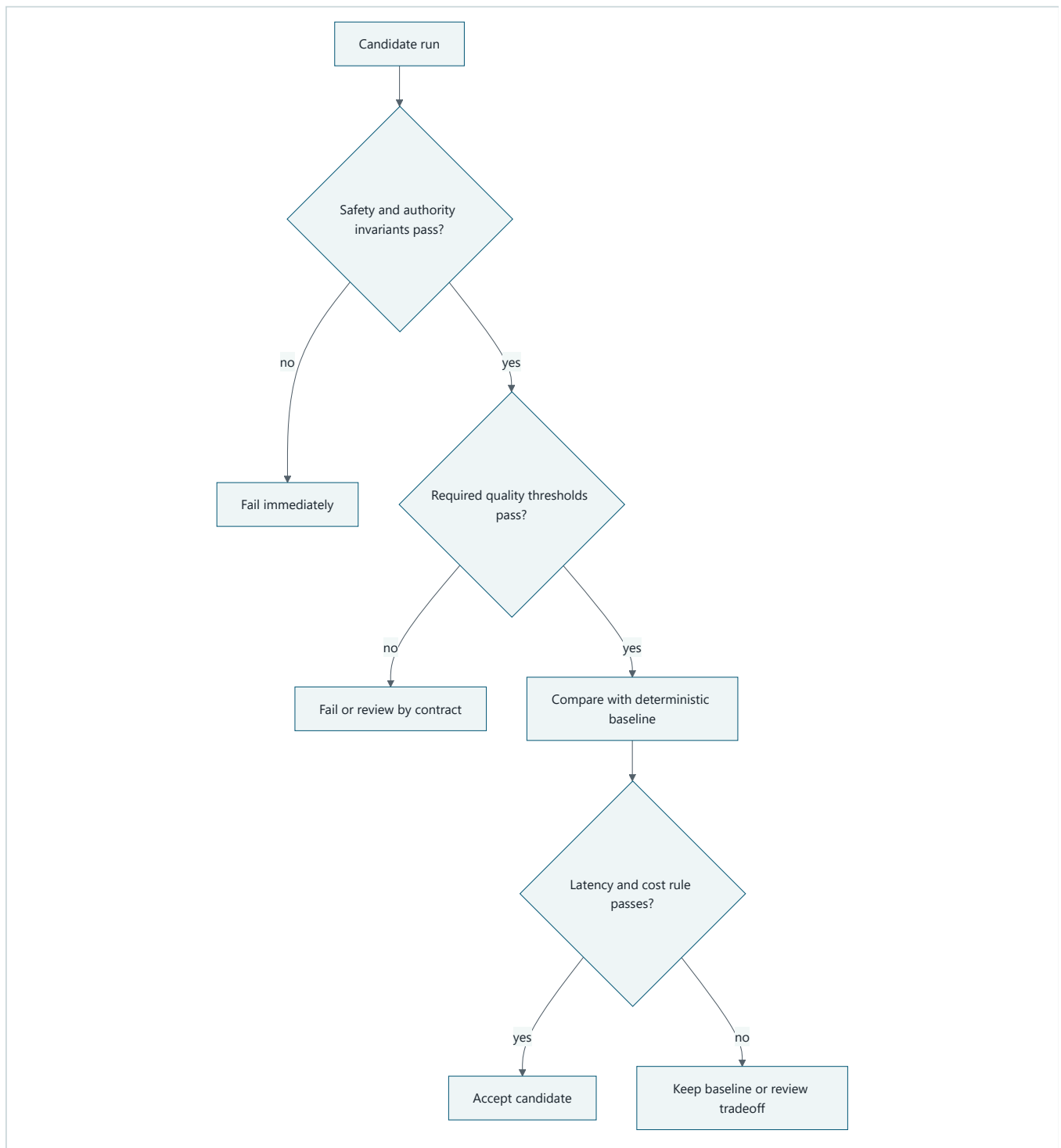
Diagram 2: invariants before tradeoffs
