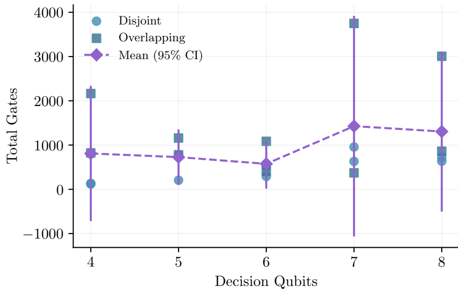
Total Gates
