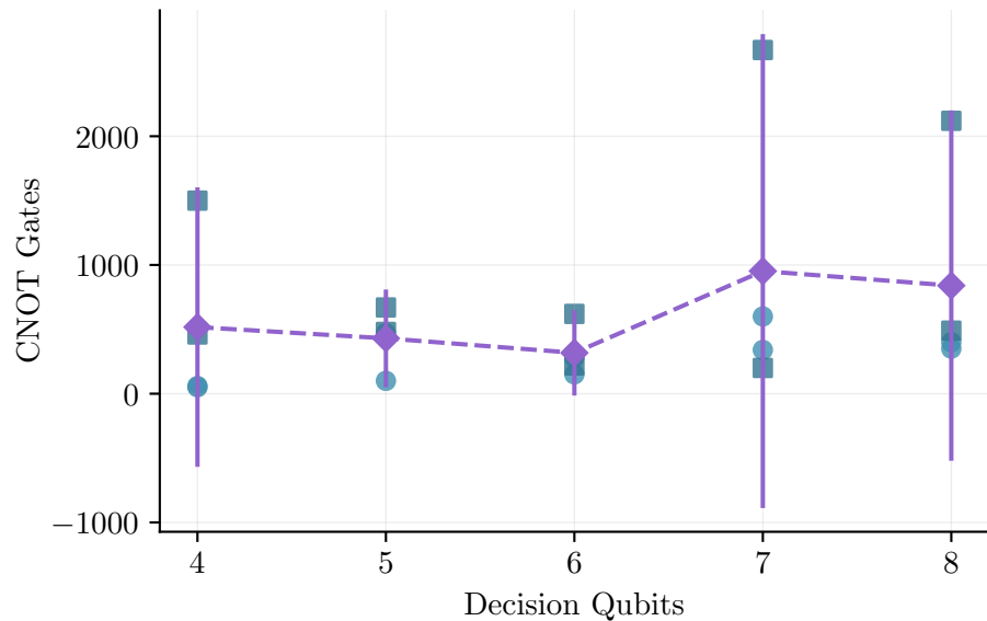
CNOT Gates
