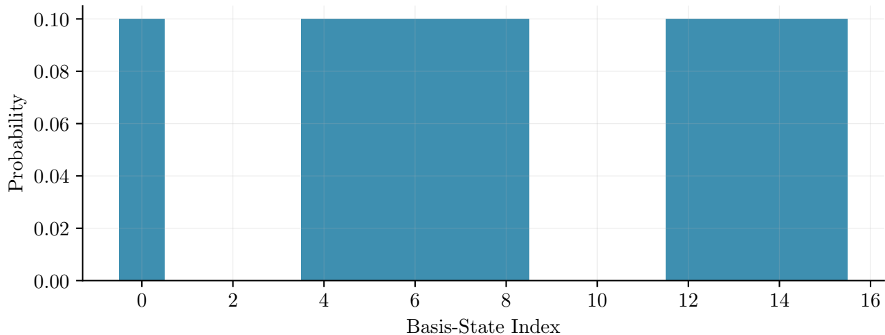
Probability Distribution: L_{\text{fid}} -x_0 - 5x_1 + 3x_2 + 3x_3 \leq 1
