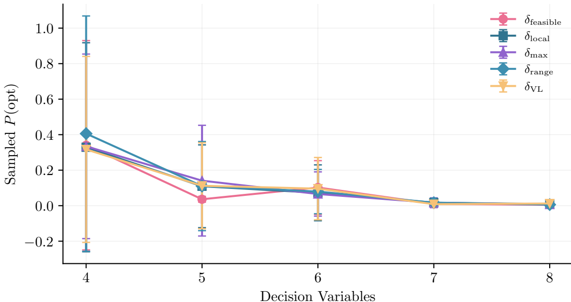
Penalty Methods by Decision Size
