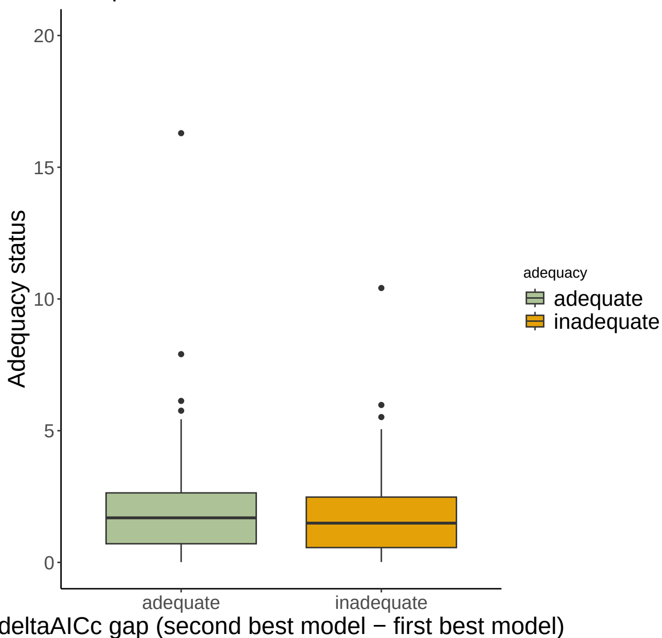
Comparison of the deltaAICc between time series which p
