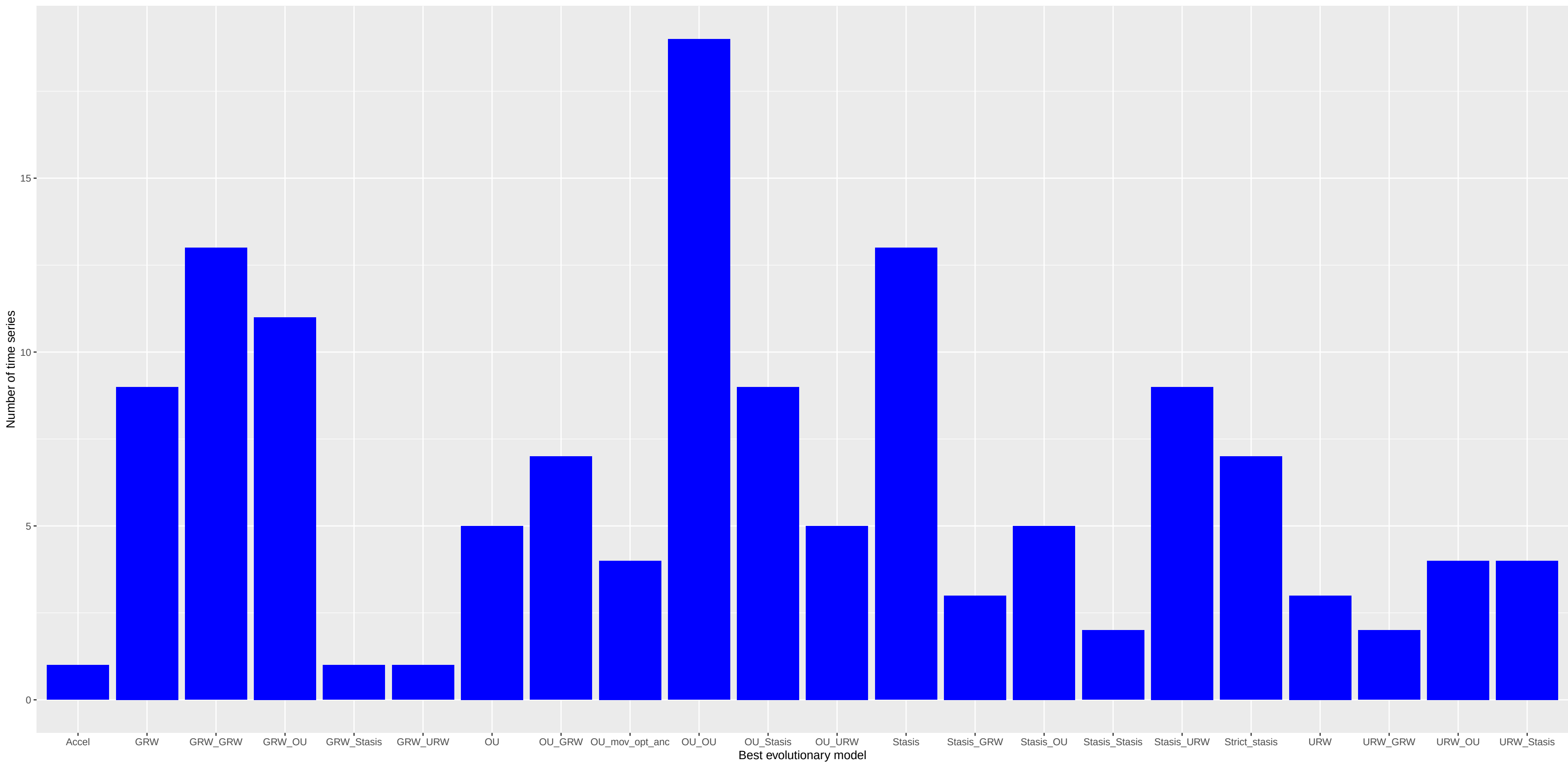
Barplot of the best model among adequate time series
