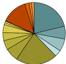
Taxa
