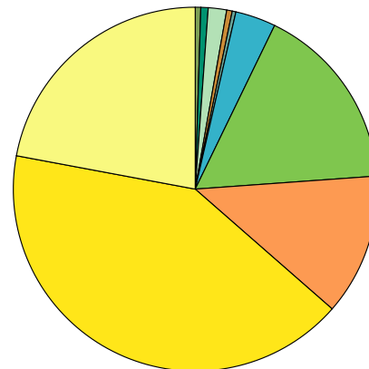
Geological period
