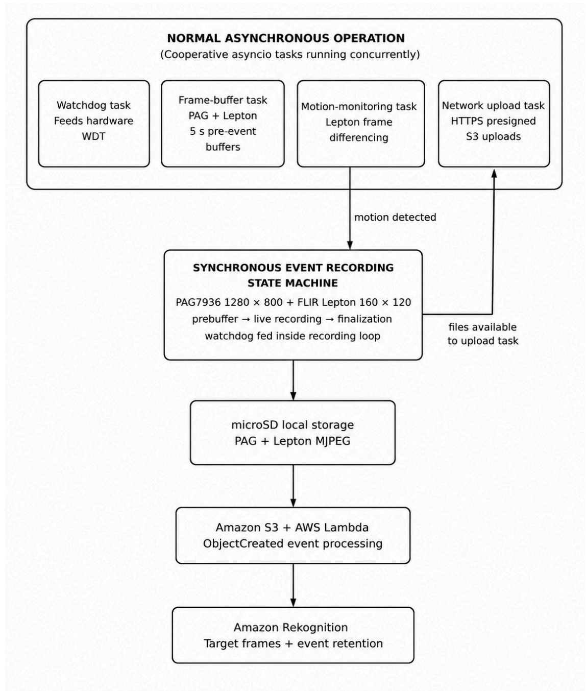
1. Figure: Embedded runtime architecture and cloud processing flow.
