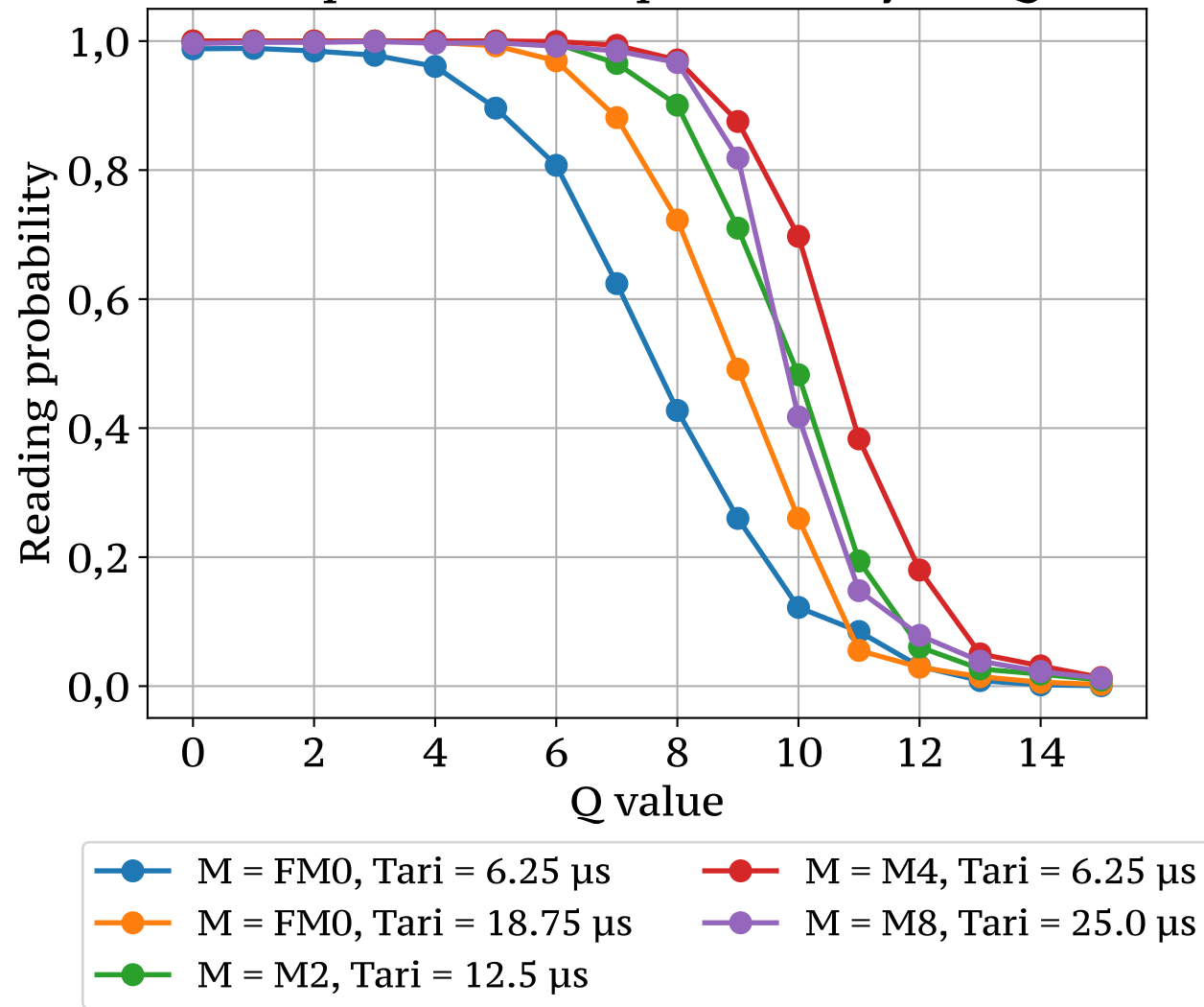
Dependence of probability on Q
