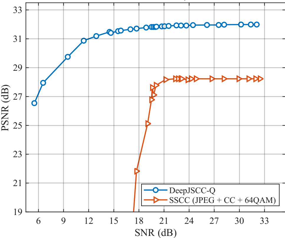
Over-the-air measurement, DIV2K 0802
