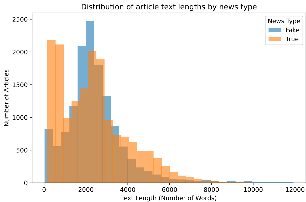
Figure 8: Distribution of article text lengths for fake and true news articles
