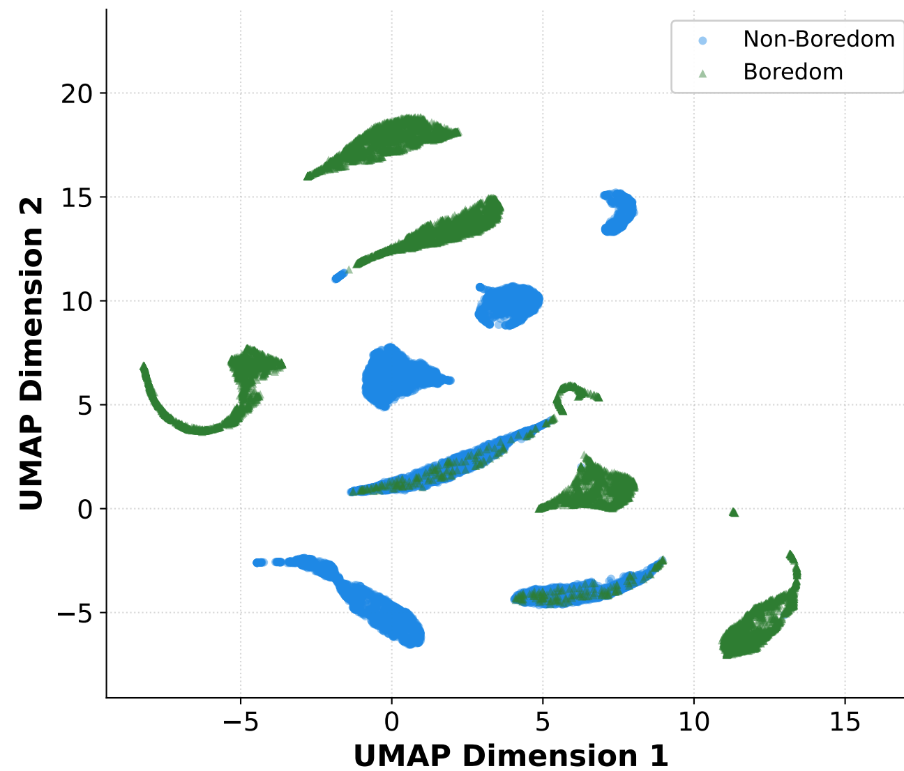
(b) Fine-Tuned LaBraM
