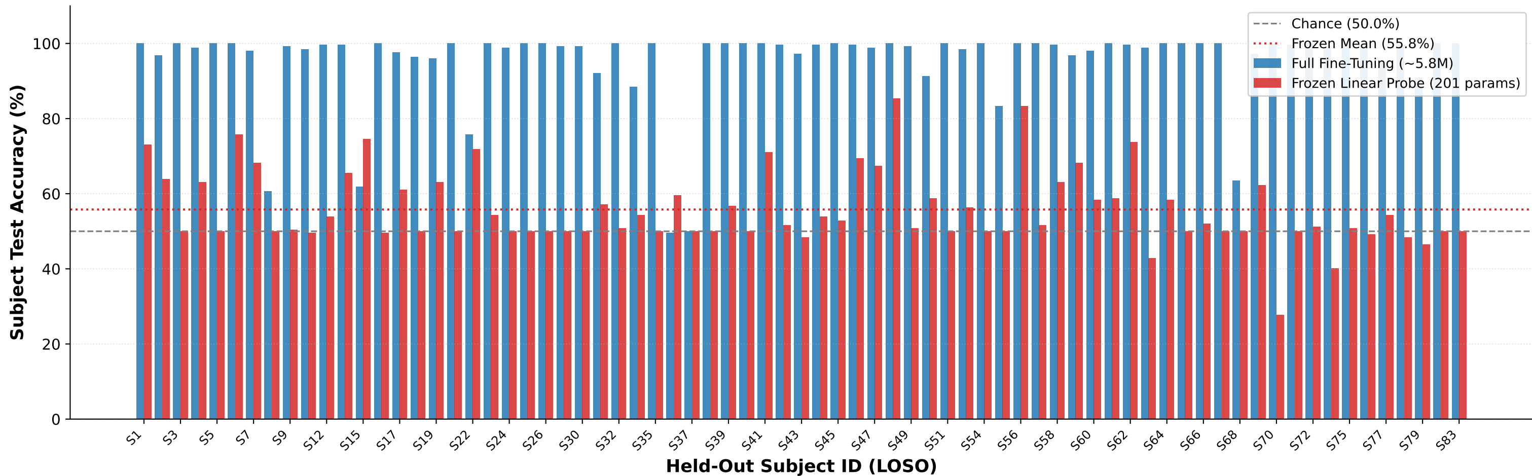
Ablation 2: Leave-One-Subject-Out (LOSO) Accuracy across 73 Subjects
