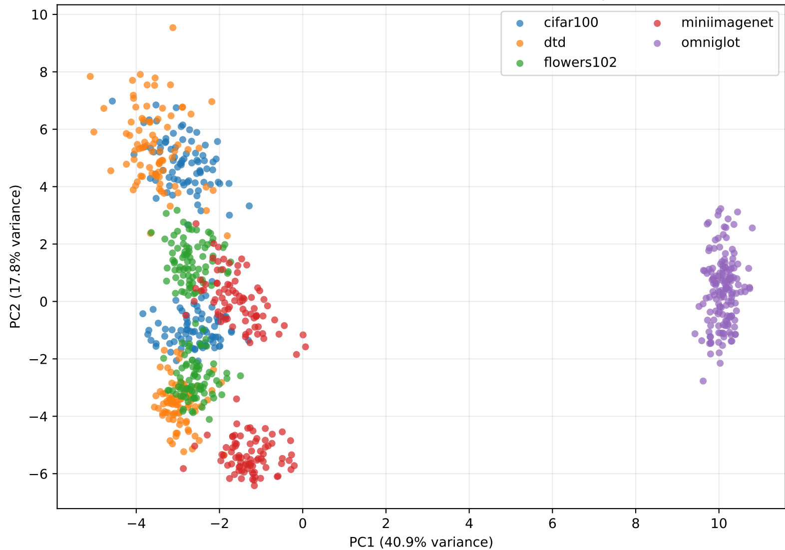
PCA of the final 64-dimensional static task descriptor
