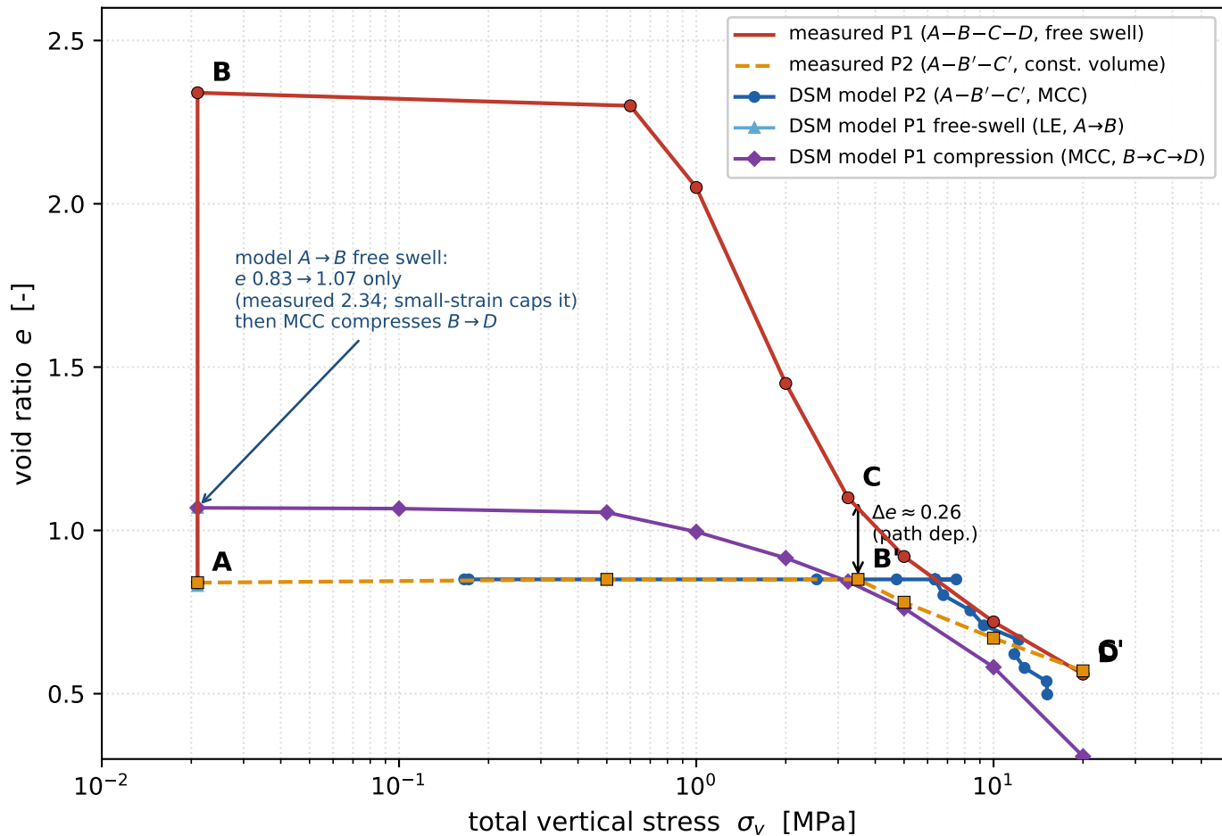
BEACON Task 3.3 granular MX-80 — both stress paths, e vs \sigma_v measured (Ferrari et al. 2022; D3.3 Tab 4-1) vs native DSM (Pi-path)
