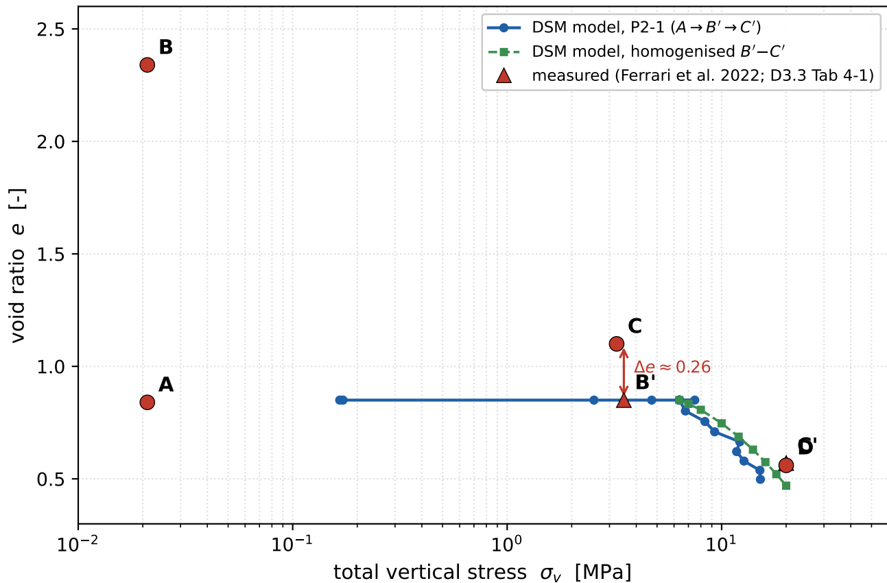
BEACON Task 3.3 — granular MX-80, e vs \sigma_v native DSM (Pi-path + MCC, k(\phi_M)^9 ) vs measured
