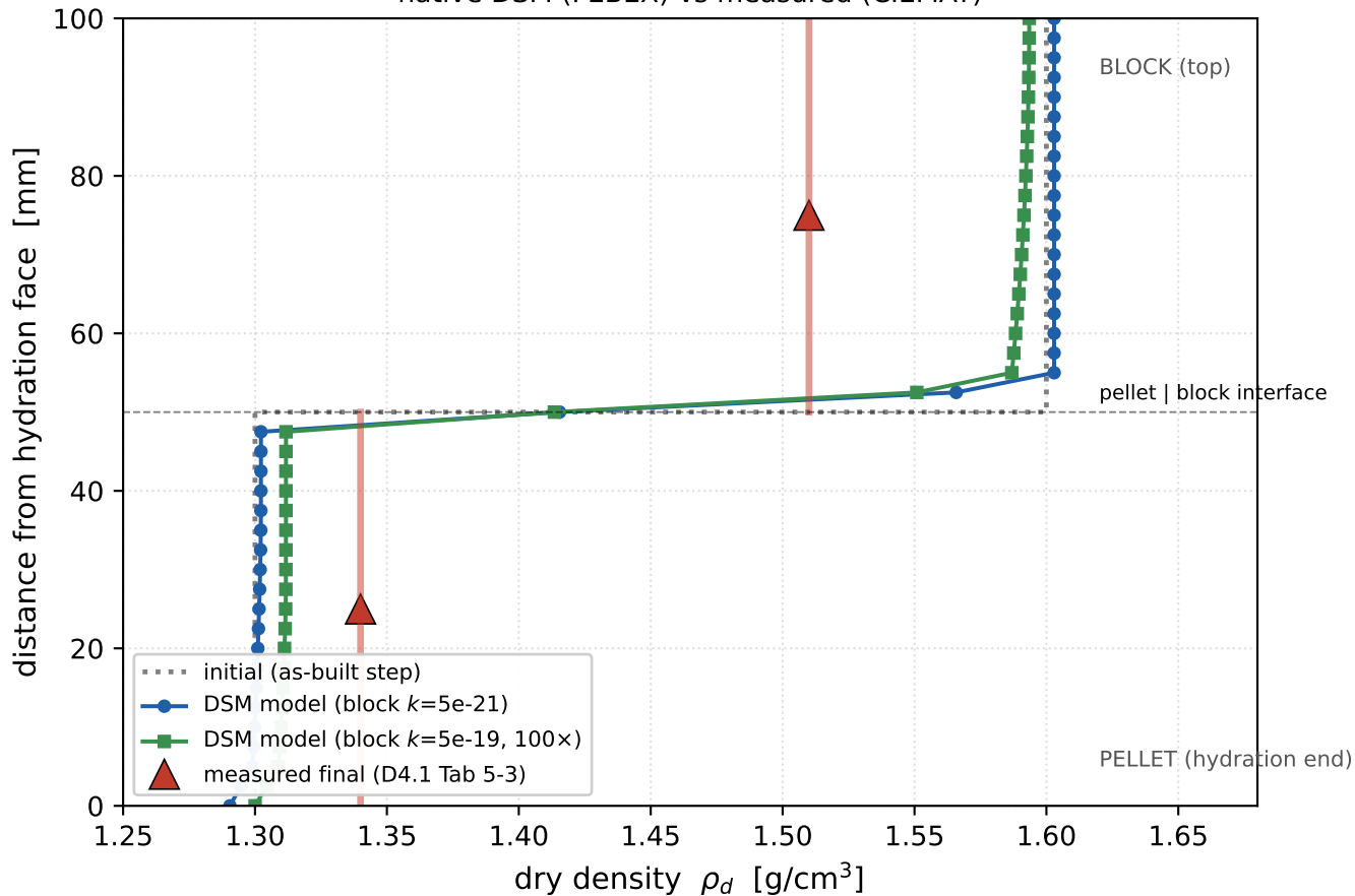
BEACON WP5.3 MGR23 — final dry-density profile native DSM (FEBEX) vs measured (CIEMAT)
