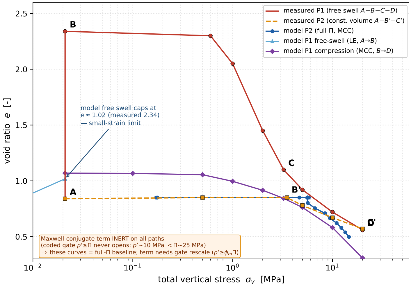
BEACON Task 3.3 granular MX-80 — both stress paths, e vs \sigma_v measured (Ferrari et al. 2022) vs model (maxwell-conjugate binary, full- \Pi ; term inert)
