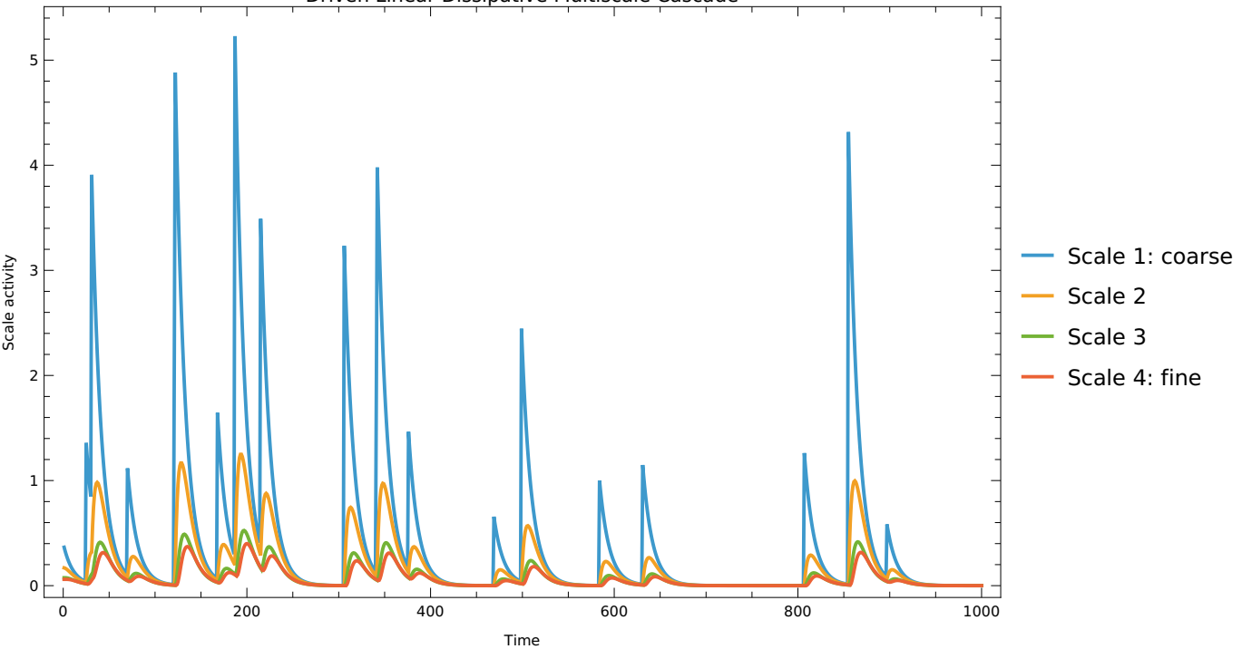
Driven Linear Dissipative Multiscale Cascade
