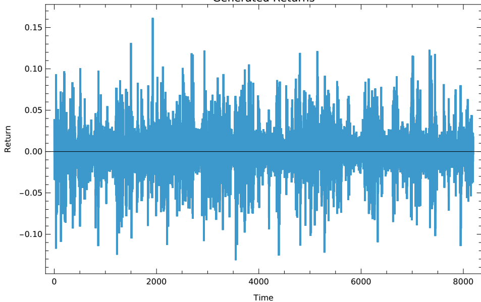
Generated Returns
