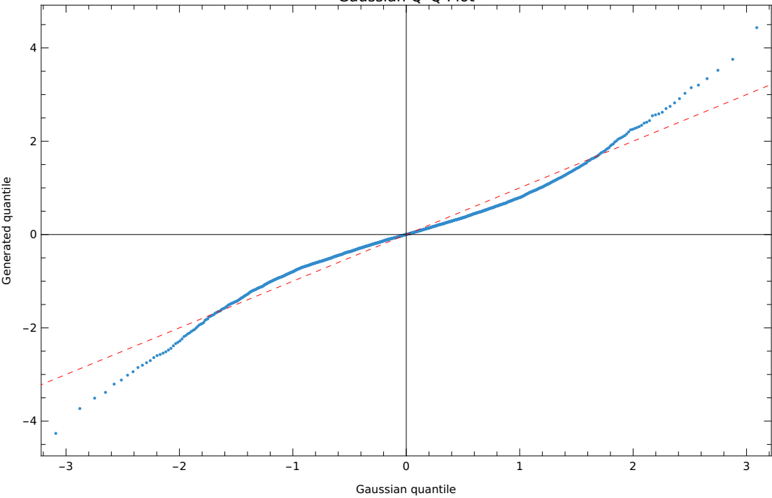
Gaussian Q-Q Plot
