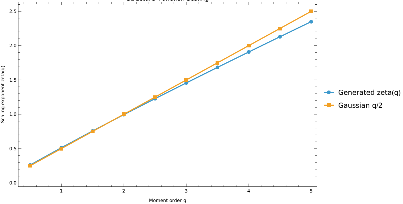
Structure-Function Scaling
