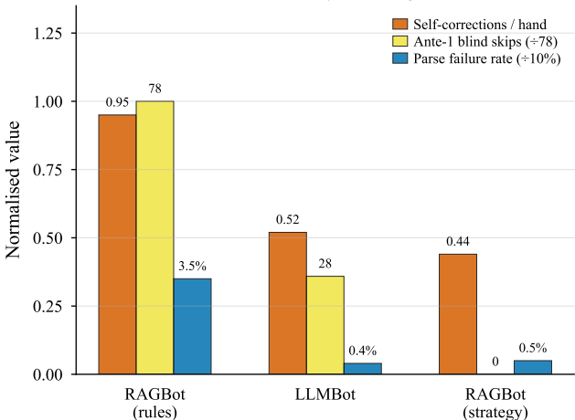
Decision Quality: LLM Agents
