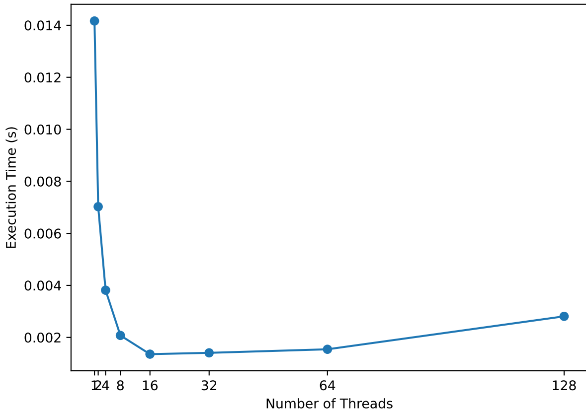
Strong Scaling (N=10,000,000)
