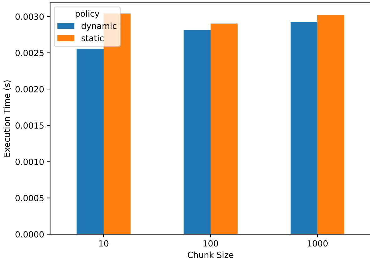
Scheduling Policies (Threads = Max, N=10,000,000)
