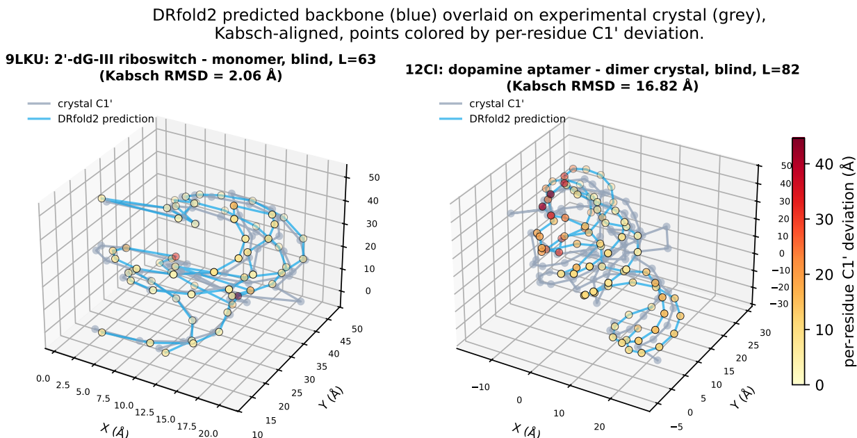
Figure 2: DRfold2 predicted backbone (blue) Kabsch-aligned to the experimental crystal C1' trace (grey), with prediction points coloured by per-residue C1' deviation. Left: 9LKU (2'-dG-III riboswitch monomer) at 2.06 Å RMSD — predicted and experimental traces are essentially super-imposable. Right: 12CI (dopamine aptamer, dimer crystal with ligand-bound interface) at 16.82 Å RMSD — DRfold2 cannot reconstitute the dimer-context conformation from monomer input.
