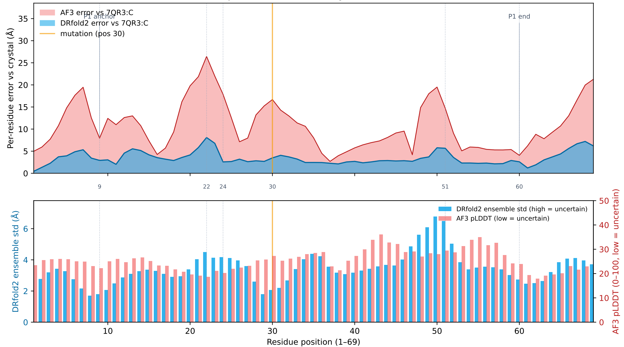
Per-residue calibration on R1108 (chimp CPEB3) vs 7QR3:C crystal
