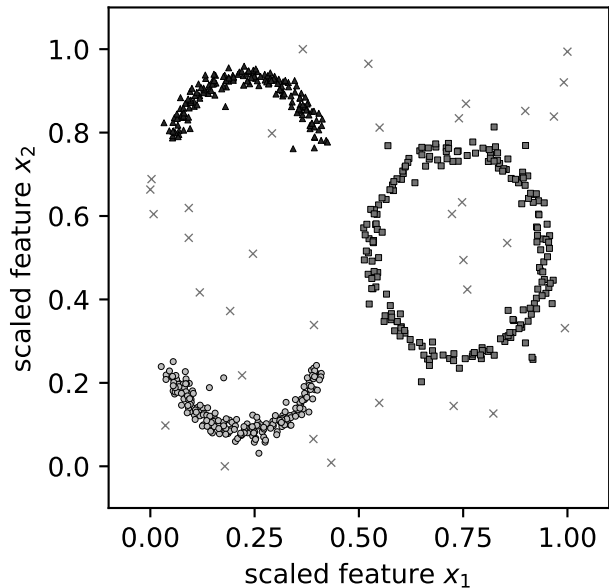
DBSCAN: shapes stay intact
