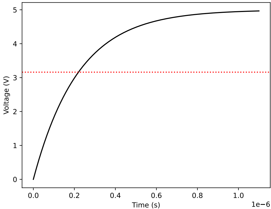
Capacitor charging ( R = 10\text{k}\Omega , C = 22\text{ pF} )
