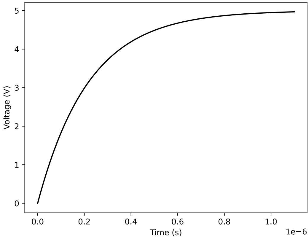
Capacitor charging
