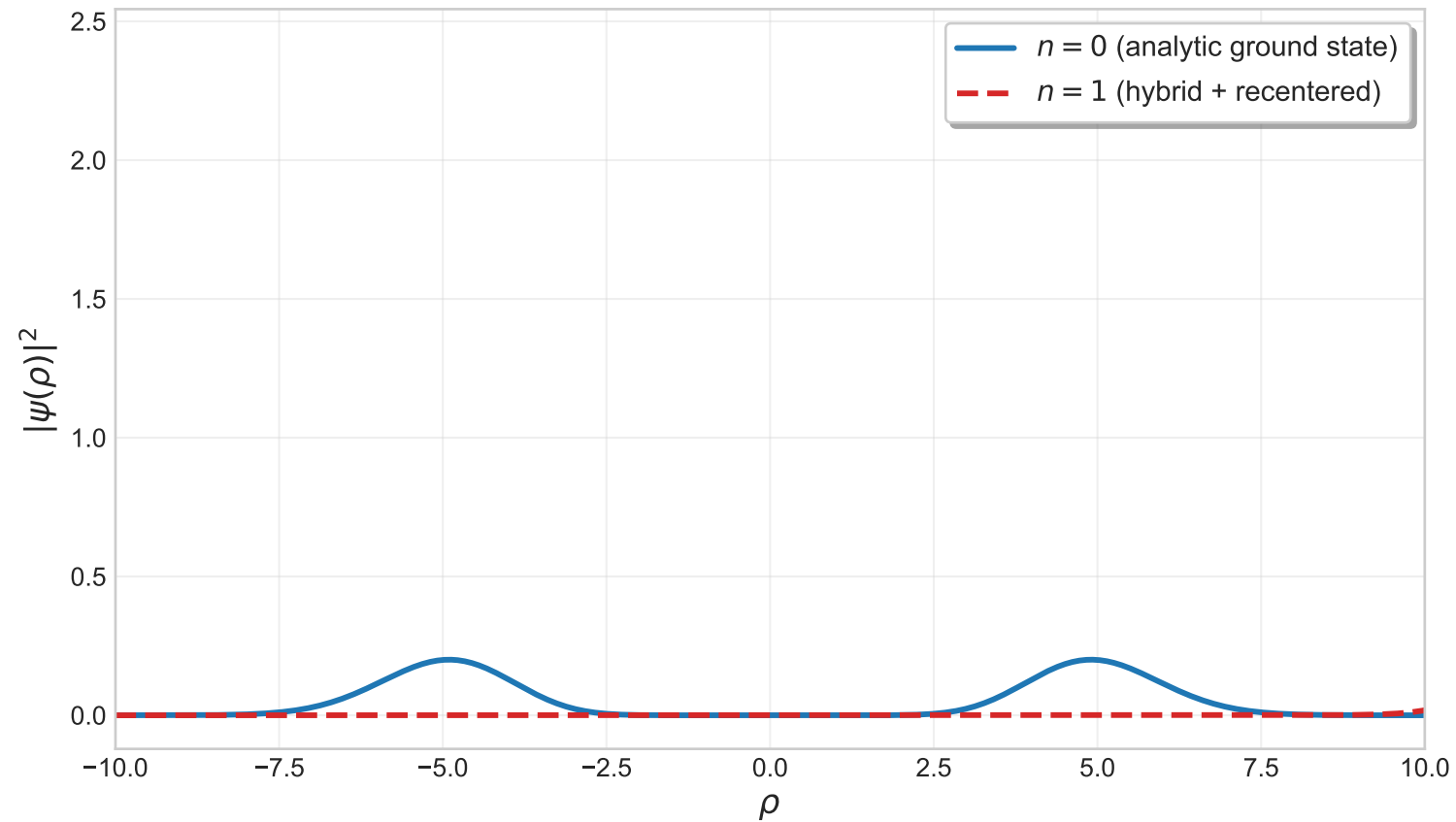
HSMT Low-Lying Spectrum: Probability Densities
