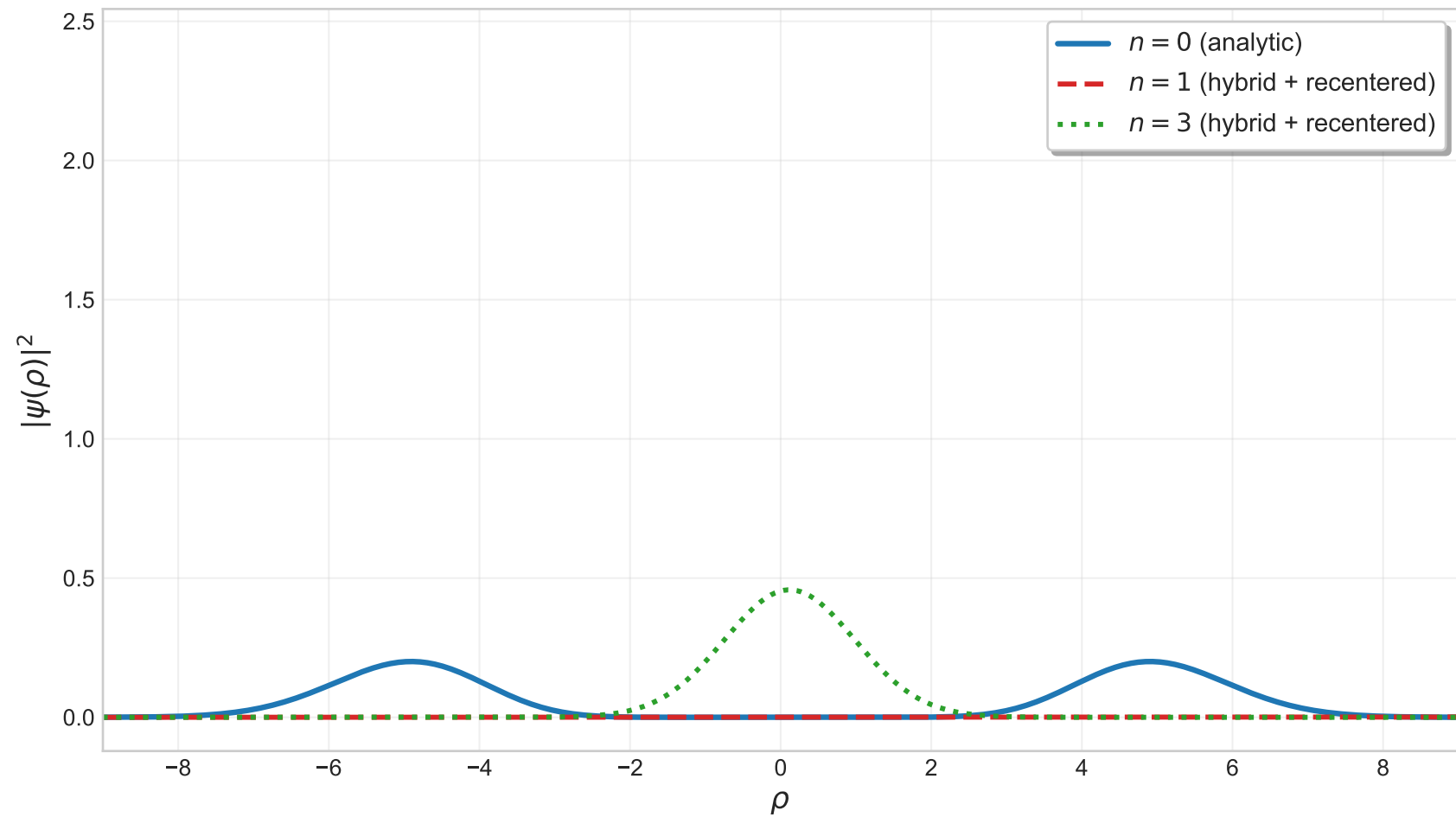
HSMT Low-Lying Spectrum: Probability Densities ( n = 0, 1, 3 )
