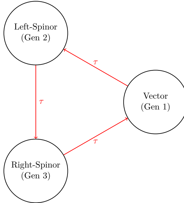
Figure 4: Triality automorphism of G_2 naturally generates the three fermion generations by cycling the vector, left-spinor, and right-spinor representations.
