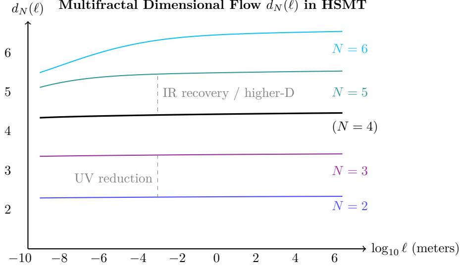
Figure 3: Effective dimension d_N(\ell) versus length scale for selected shells. Lower shells show strong reduction at short distances (quantum regime), while higher shells exhibit elevated dimension at large scales (contributing to apparent cosmic acceleration).
