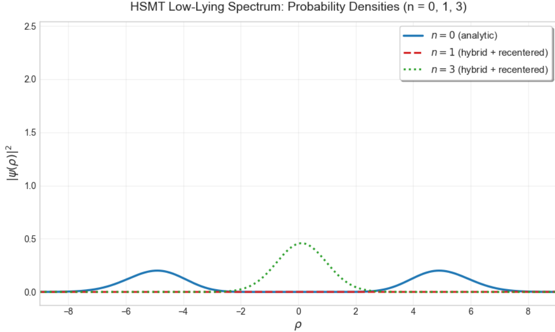
Figure 2: Probability densities for the ground state ( n = 0 , analytic) and two excited states ( n = 1 and n = 3 ) obtained via the hybrid hypergeometric reconstruction + recentering method. The improvement in centering for the excited states is clearly visible.
