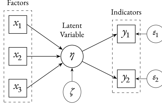
Figure 1 · Path Diagram
