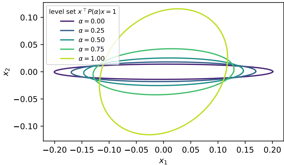
Parameter-dependent Lyapunov function P(\alpha) = \Gamma_1(A(\alpha))^\top P_j \Gamma_1(A(\alpha)) from a single P_j ( N = 1 )
