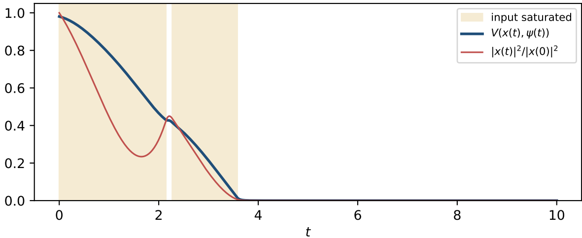
Jet Lyapunov function along a trajectory starting on the boundary of its estimate
