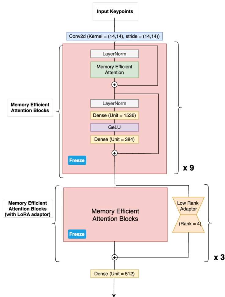
Figure 2: Spatial-model schematic. The pretrained DINOv2-style backbone is largely frozen, while selected later blocks are adapted through LoRA modules.
