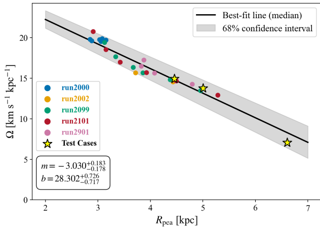
Figure 5. Bayesian linear regression of the relation between peanut length ( R_{\text{pea}} ) and bar pattern speed ( \Omega ). Colored circles show post-buckling snapshots for models run2000 (blue), run2002 (orange), run2099 (green), run2101 (red), and run2901 (pink). Yellow stars indicate selected test cases. The black line corresponds to the median best-fit relation, with the gray band showing the 68% confidence interval. The inset box gives the slope and intercept with 1\sigma uncertainties.
