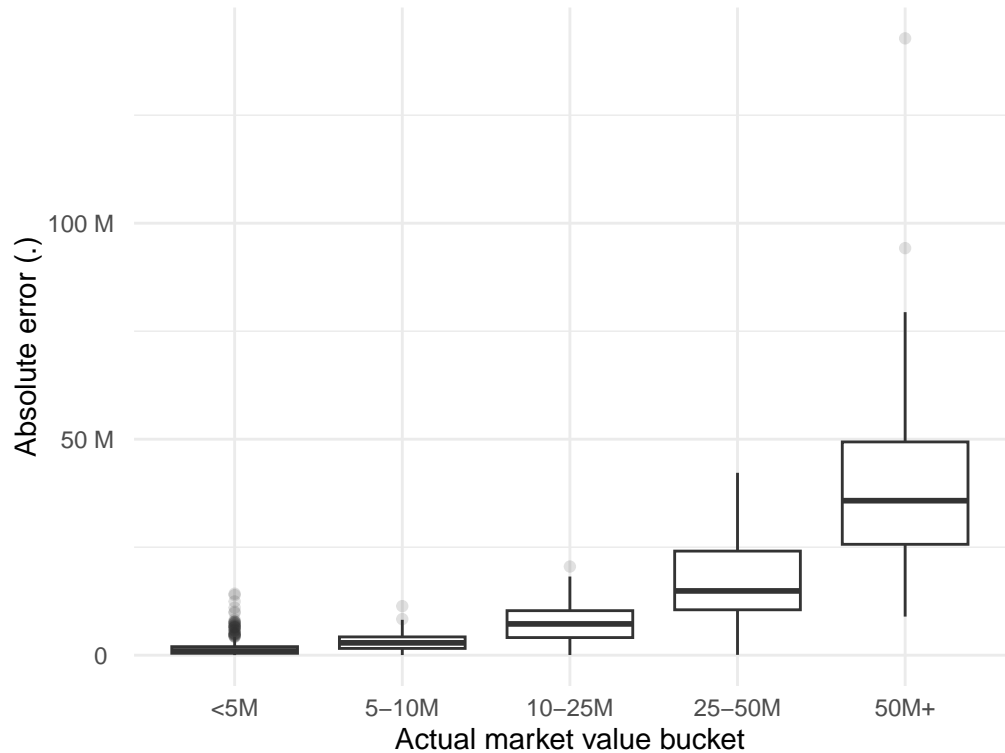
Prediction error by market value bucket (2024–25)
