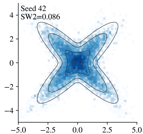
Conditional Stein estimator
