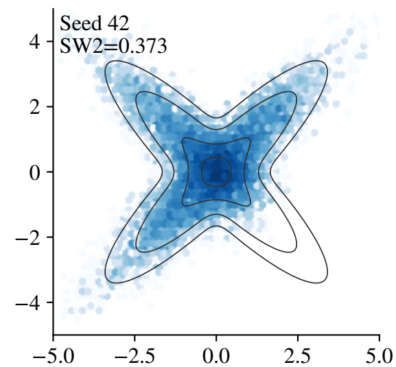
Conditional variance floor 0.2
