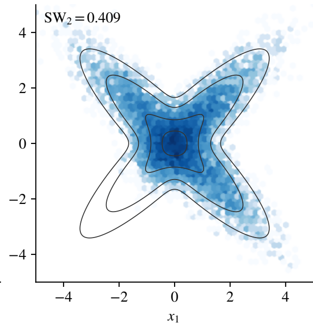
Conditional variance floor 0.2
