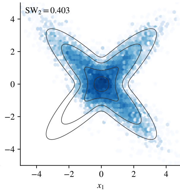
Conditional Stein estimator
